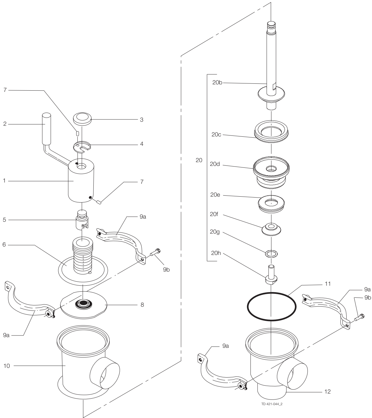
Alternative stem seal
