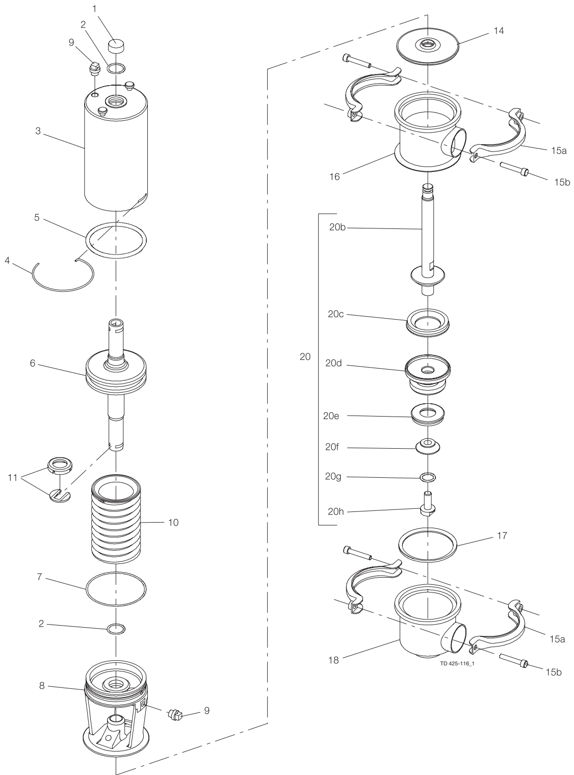
Alternative stem seal
