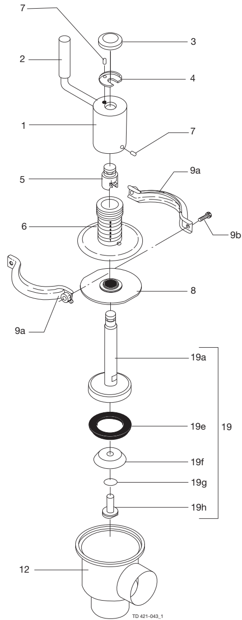
Alternative stem seal
